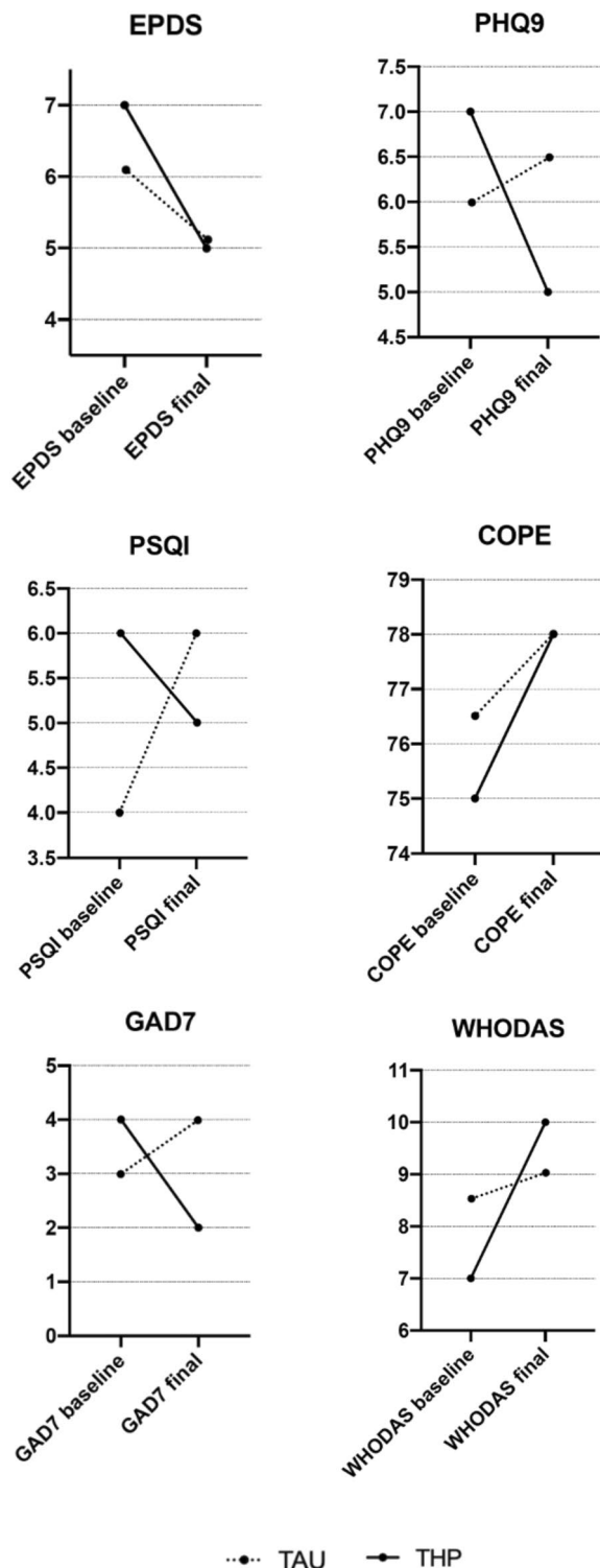
Fig. 2 Outcome measures pre to postintervention. Abbreviations: THP Thinking Healthy Programme, TAU Treatment as Usual
