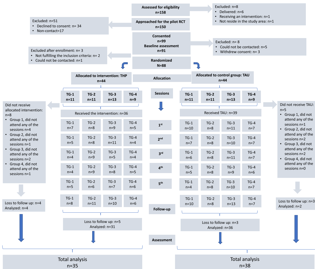
Fig. 1 Participant Flow Diagram. Abbreviations: THP Thinking Healthy Programme, TAU Treatment as Usual
